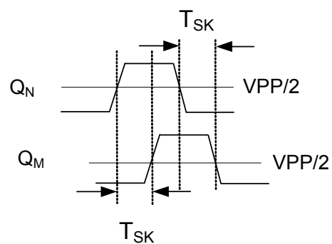
Output-Output Skew
