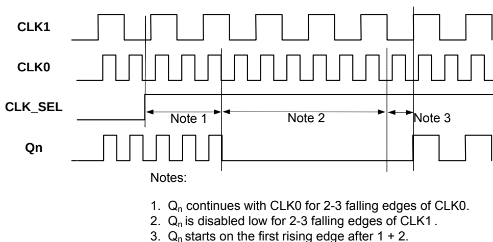
Figure 6. Glitchless Input Clock Switch
