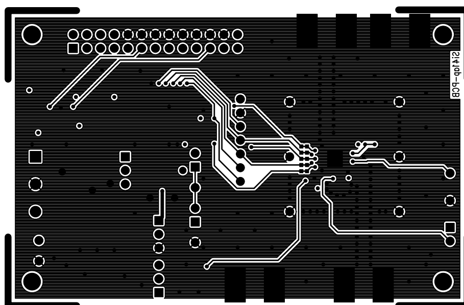
Figure 40. Si4135M Solder
