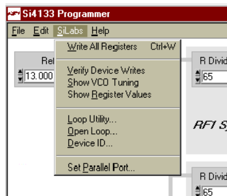
Figure 5. SiLabs Menu
