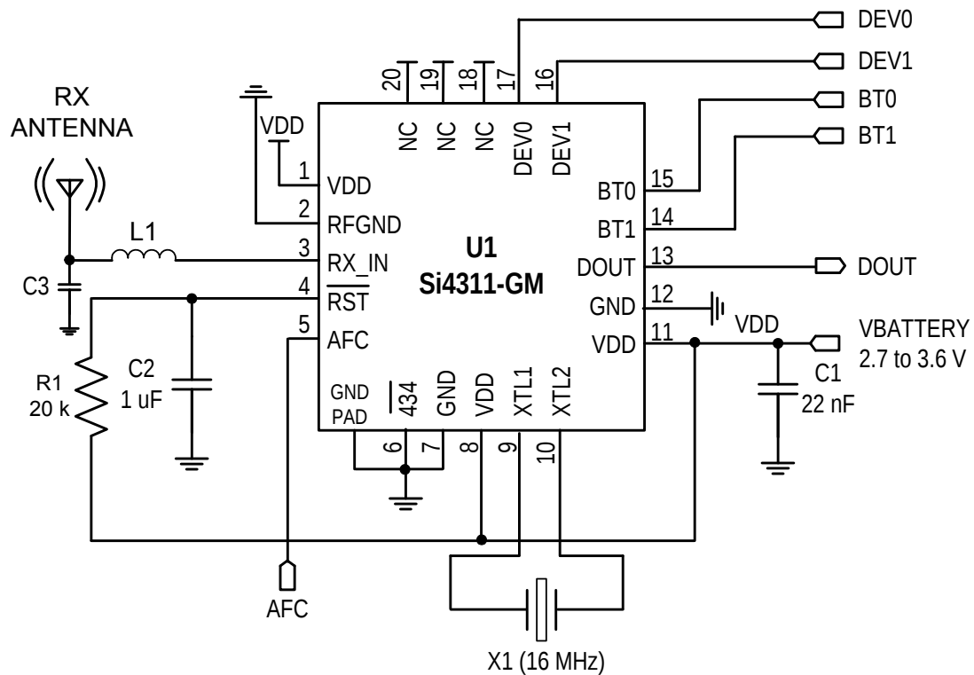
Figure 2. Si4311 FSK 433.92 MHz Application Schematic
