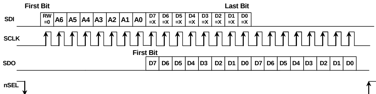
Figure 6. SPI Timing—Burst Read Mode
