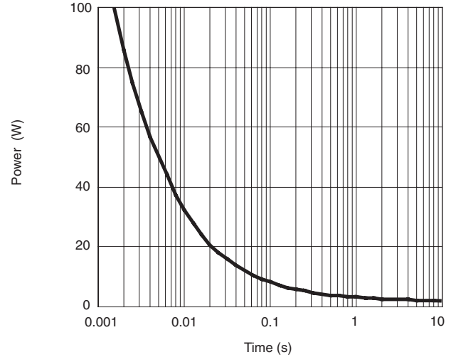
Single Pulse Power vs. Junction-to-Ambient
