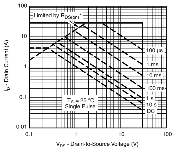
Safe Operating Area, Junction-to-Ambient * V_{DS} > minimum V_{GS} at which R_{DS(on)} is specified
