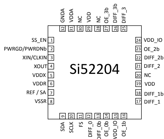
Figure 9.3. 32-pin QFN
