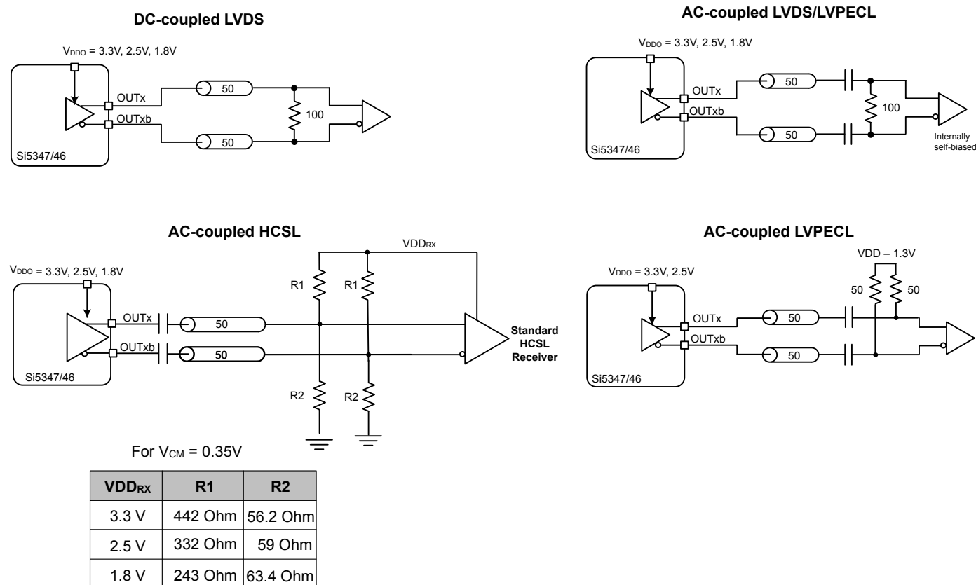
Figure 3.15. Supported Differential Output Terminations
