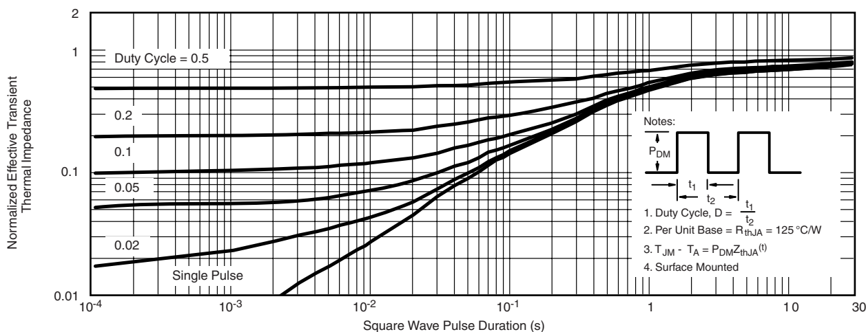
Normalized Thermal Transient Thermal Impedance, Junction-to-Ambient
