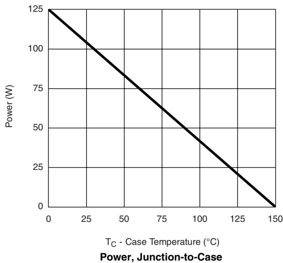
Power, Junction-to-Case
