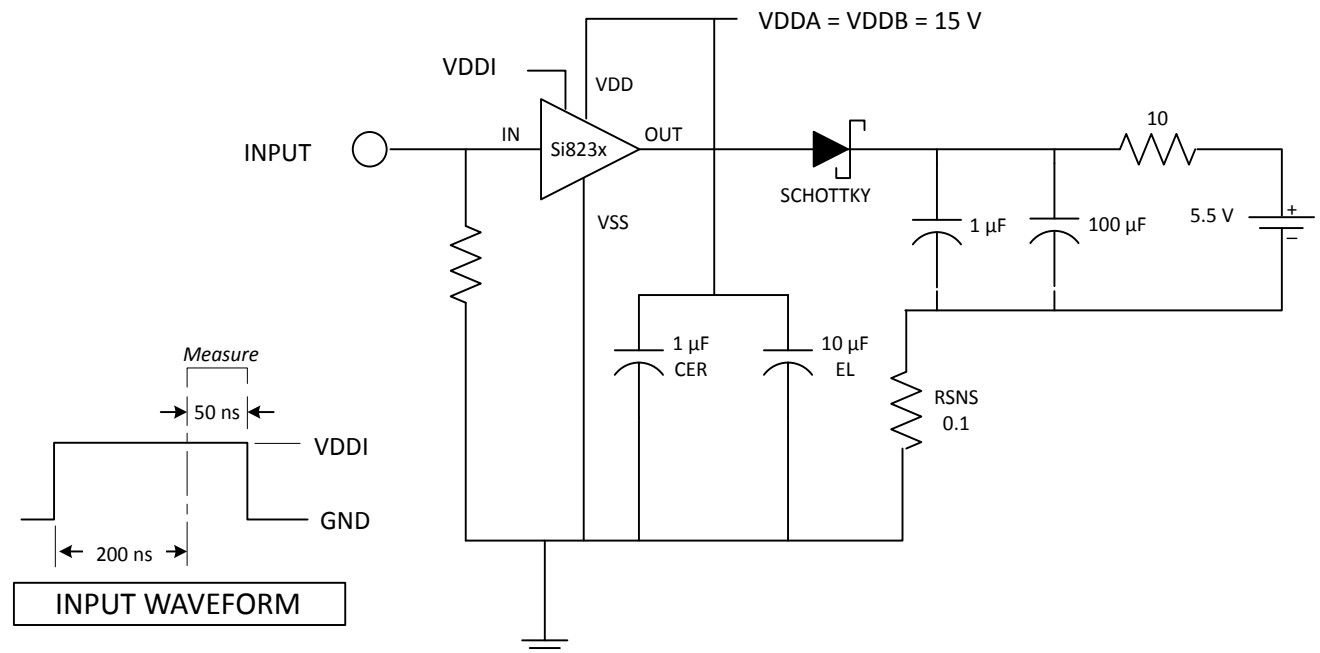
Figure 4.2. IOH Source Current Test Circuit
