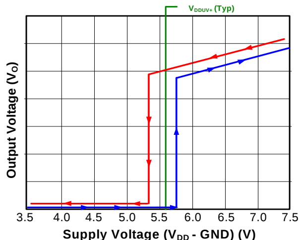
Figure 11. Si826xxAx UVLO Response (5 V)
