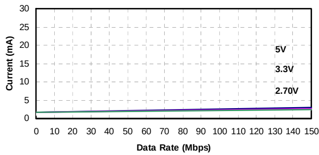
Figure 14. Si8423 Typical V_{DD1} Supply Current vs. Data Rate 5, 3.3, and 2.70 V Operation
