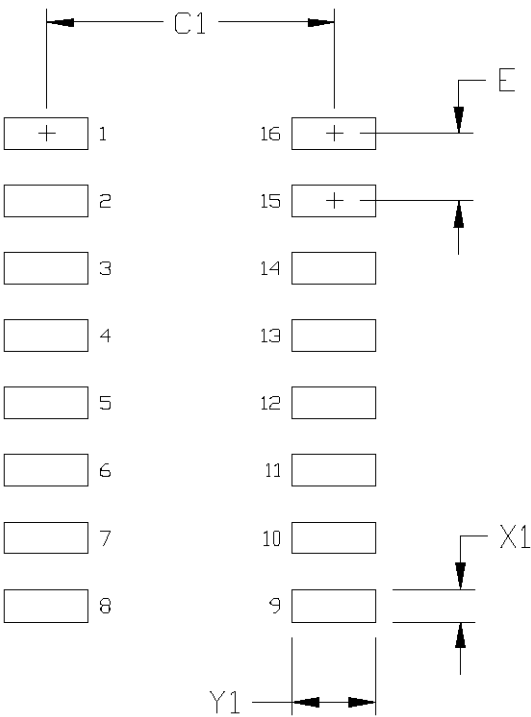
Figure 10.1. 16-Pin Narrow Body SOIC PCB Land Pattern
