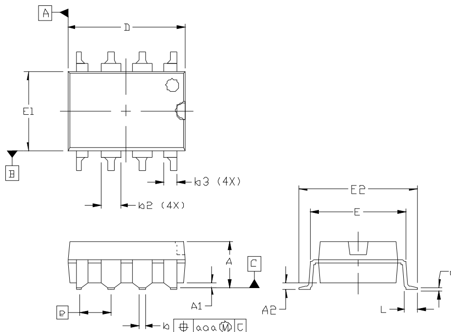
Figure 13. DIP8 Package
