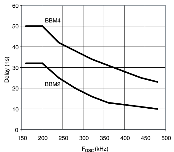
Figure 9. Reduction in BBM2 and BBM4 Si9122E BBM vs. F_{osc} ; V_{IN} = 50 \text{ V} , V_{CC} = 10 \text{ V} , BST = 60 \text{ V} , LX = 50 \text{ V} , V_{EP} = 0 \text{ V}
