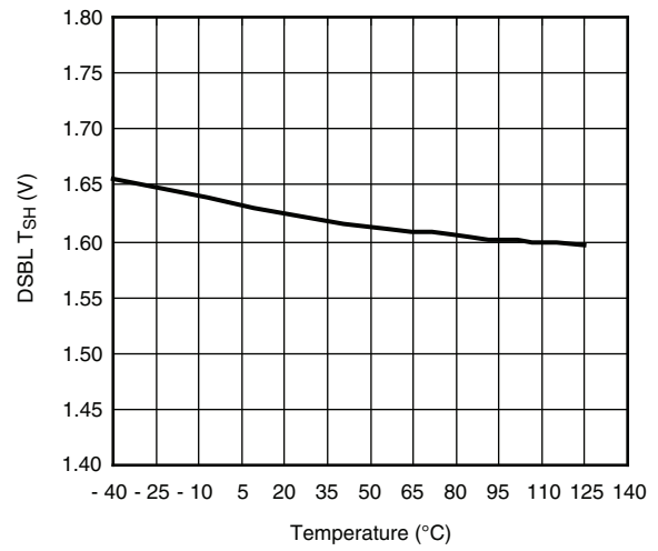
DSBL Rising Threshold (V) vs. Temperature (°C) V_{CIN} = V_{DRV} = 5\text{ V}
