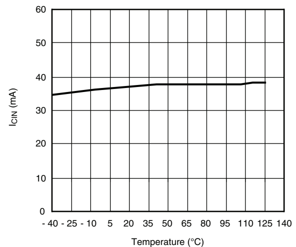
I_{CIN} + I_{DRV} (mA) vs. Temperature at Frequency = 1 MHz D = 10\% , V_{CIN} = V_{DRV} = 5\text{ V}
