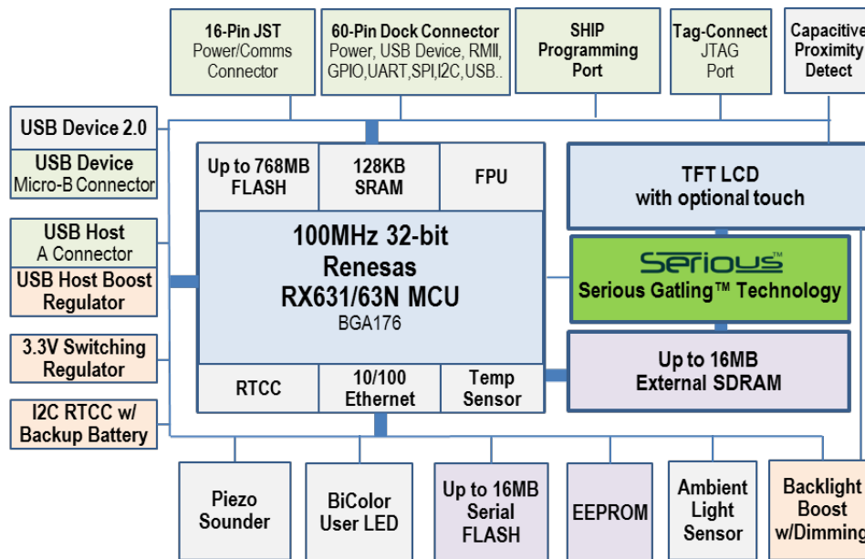
SIM231 Hardware Block Diagram
