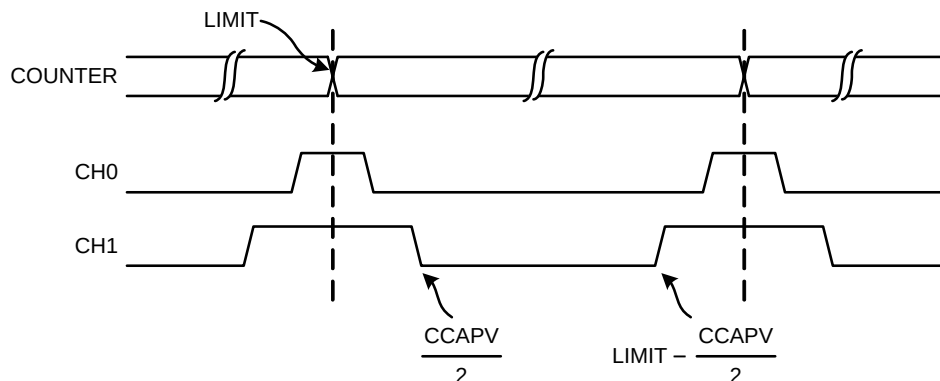
Figure 29.6. Multiple Center-Aligned PWM Channels
