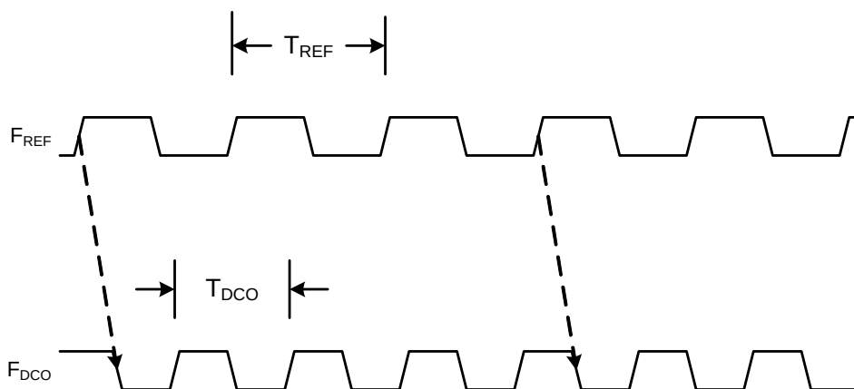
Figure 30.3. Frequency-Lock Mode
