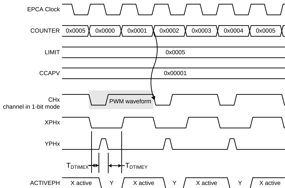
Figure 28.13. Example N-bit Edge-Aligned PWM Timing Diagram
