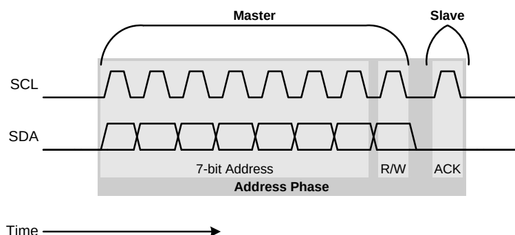
Figure 22.4. I2C 7-bit Address Phase
