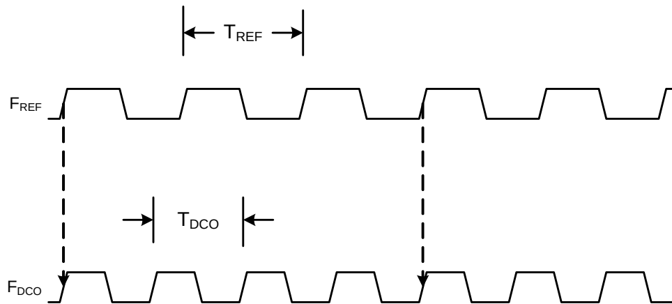
Figure 30.4. Phase-Lock Mode
