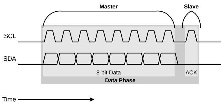
Figure 22.7. Single Byte I2C Write Data Phase
