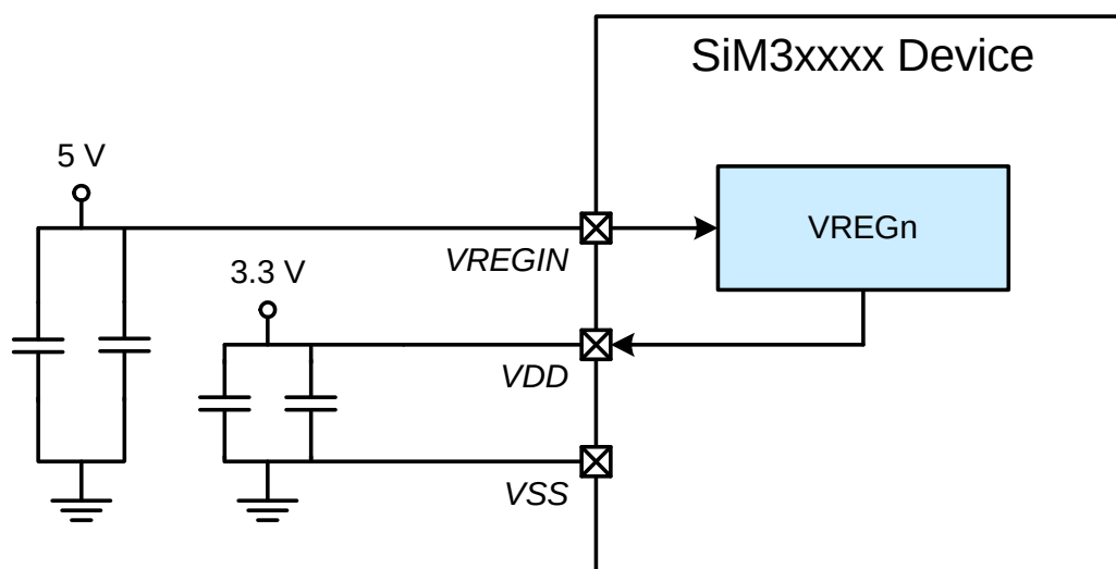
Figure 41.2. Typical Voltage Regulator Connection Diagram (Normal, Sleep, or Suspend Modes)
