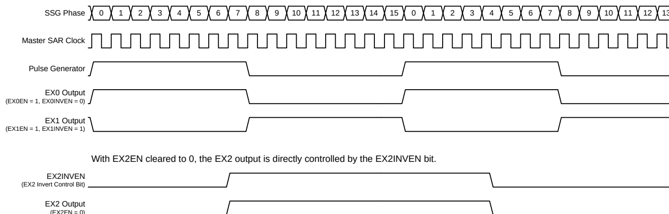
Figure 34.3. Timing Effects of the EXnEN and EXnNIVEN Bits (SSEL = 0)
