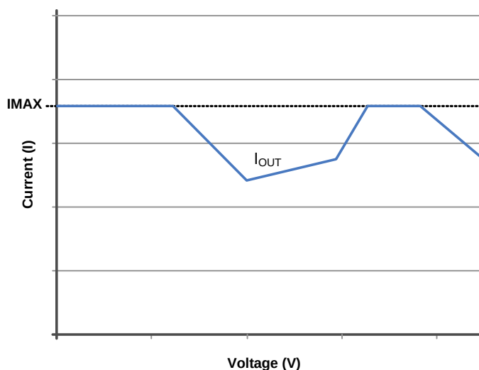
Figure 20.9. Regulator Current Limiting
