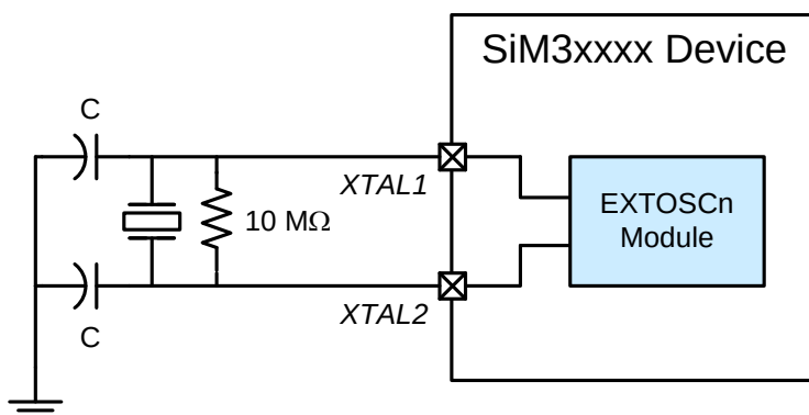
Figure 19.2. External Crystal Oscillator Configuration
