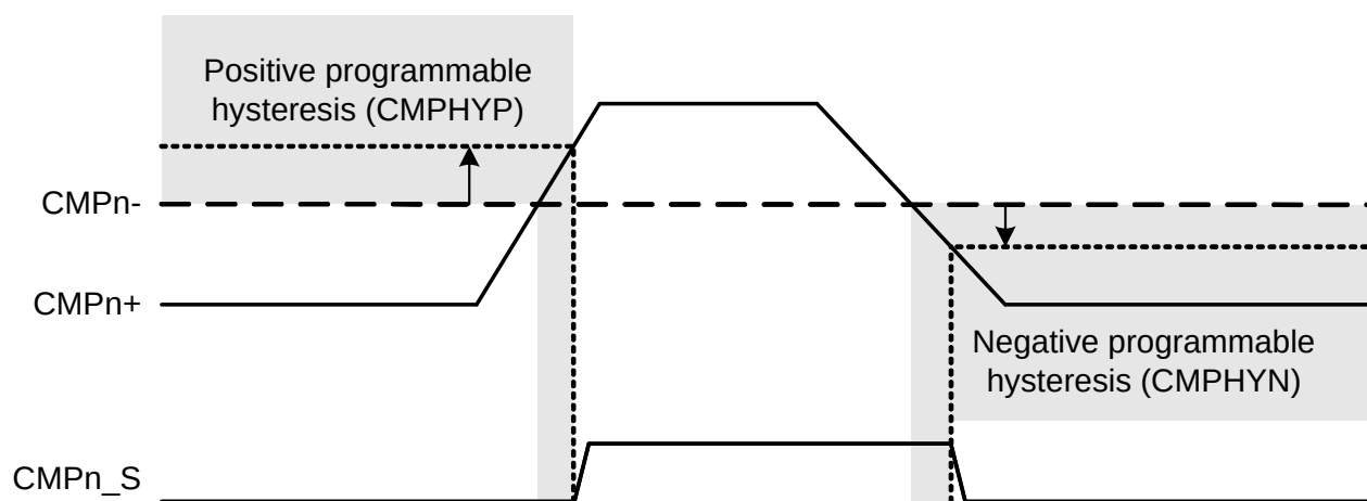
Figure 14.7. Comparator Hysteresis
