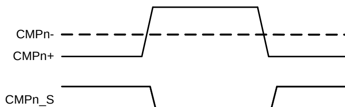
Figure 14.6. Output Configurations
