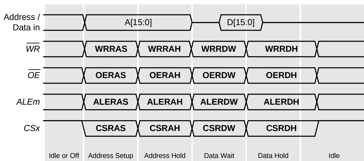
Figure 18.11. EMIF Multiplexed Transaction Timing (16-bit Bus, Read)
