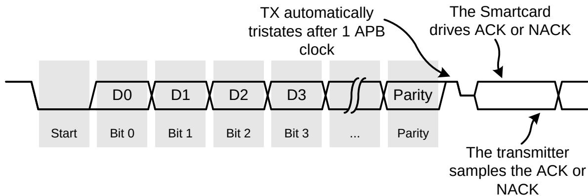
Figure 37.5. Smartcard Transmit Signalling
