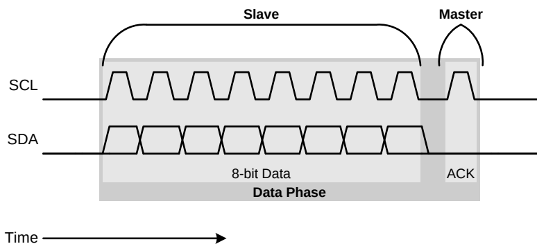
Figure 22.6. Single Byte I2C Read Data Phase
