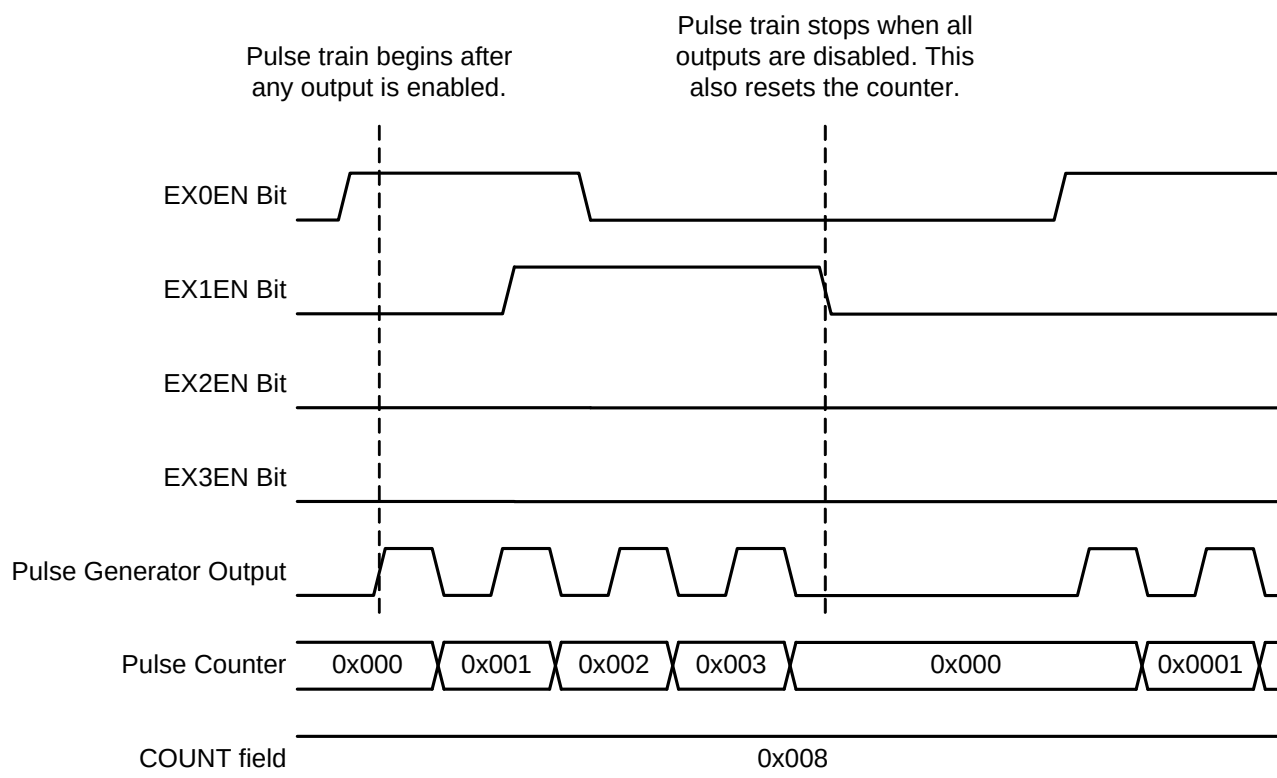
Figure 34.5. Pulse Counter Operation with Multiple Channels
