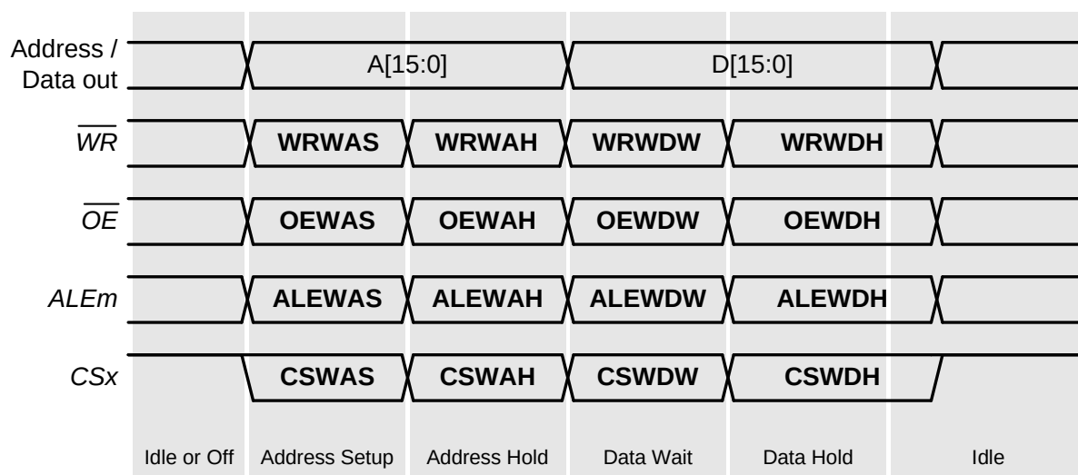
Figure 18.10. EMIF Multiplexed Transaction Timing (16-bit Bus, Write)
