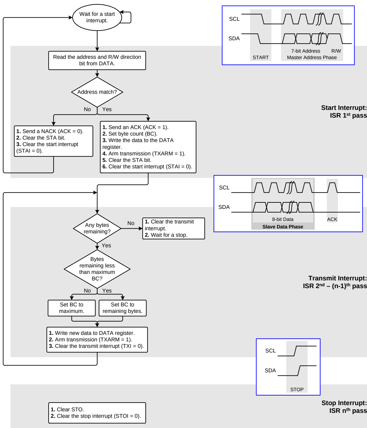
Figure 22.13. Slave Read Flow Diagram (7-bit Address)
