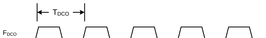
Equation 30.1. Average DCO Output Frequency
