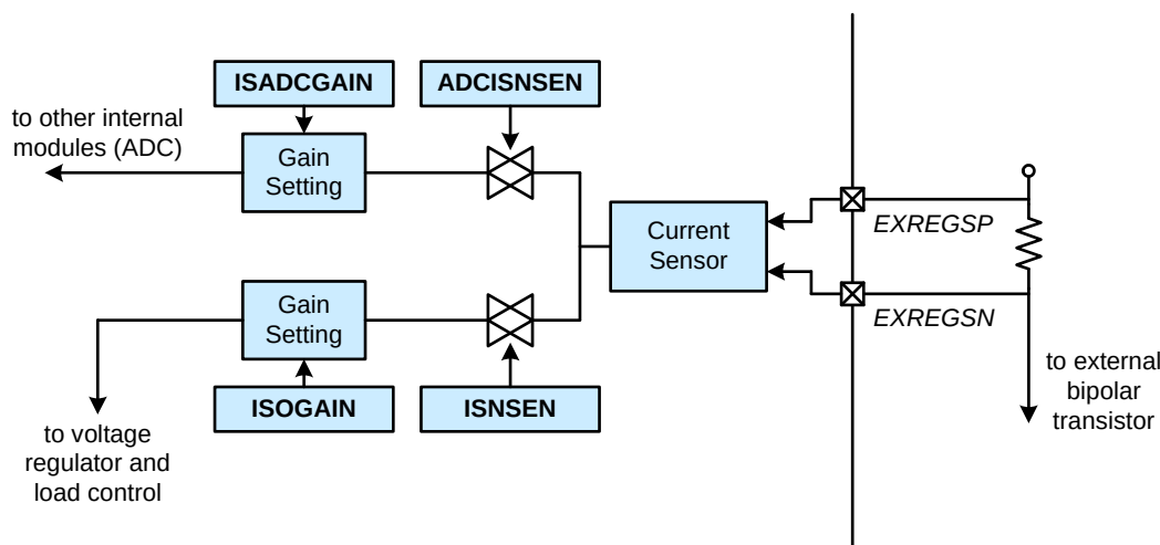
Figure 20.5. Current Sensing
