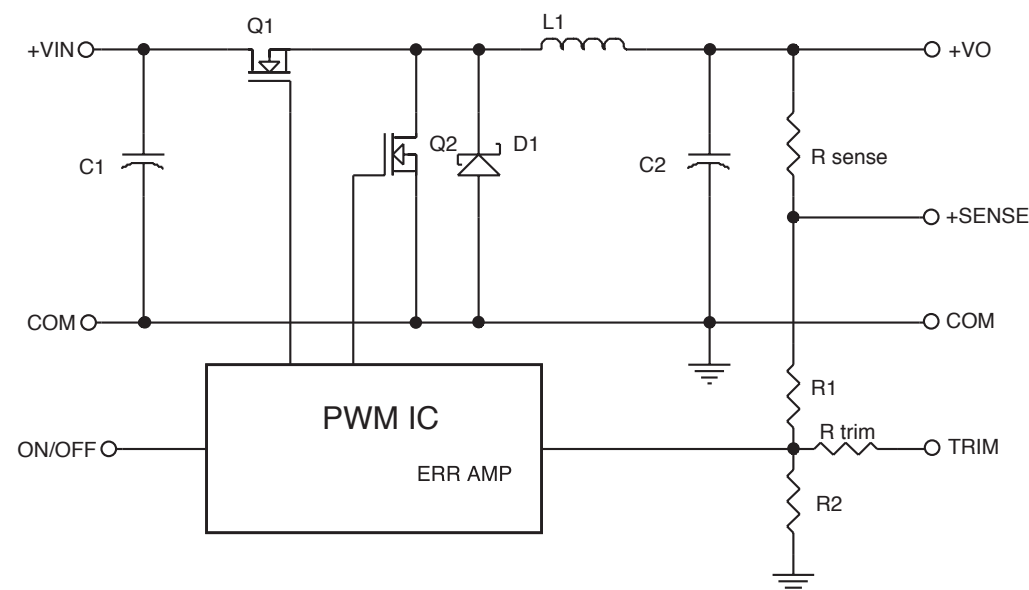
Figure 1. Simplified Schematic
