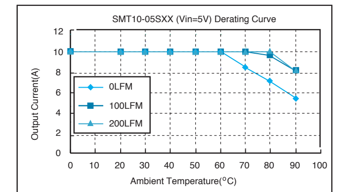
Figure 3. Typical Power De-rating for 5V IN
