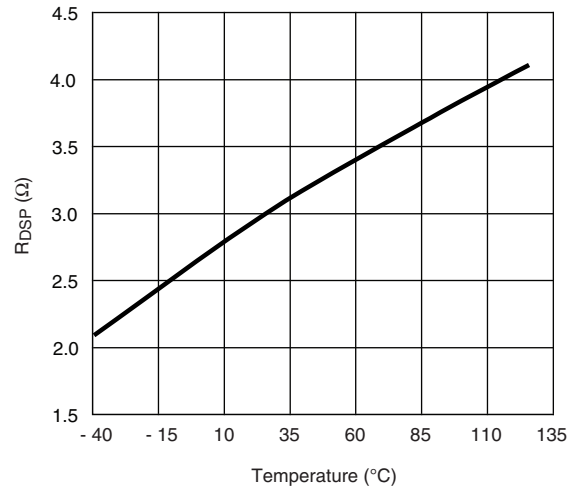
DL R_{DSN} vs. Temperature
