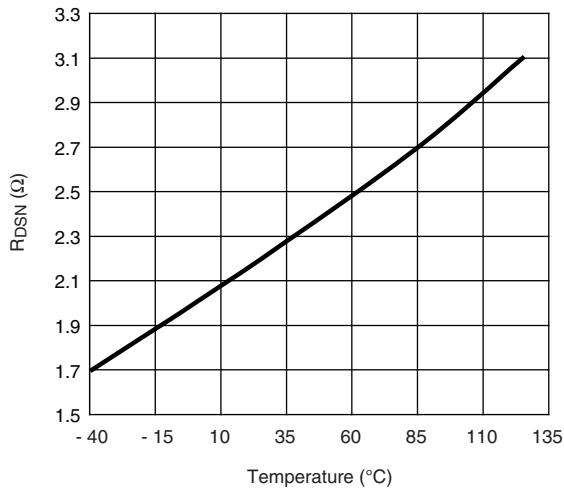
DL R_{DSN} vs. Temperature
