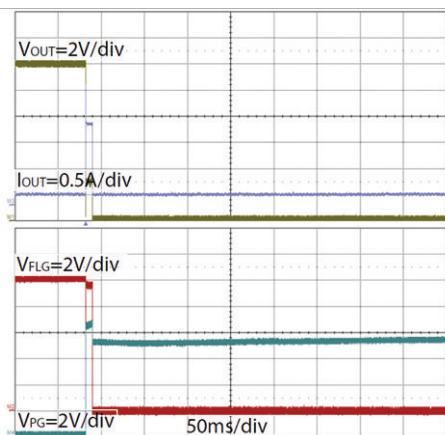
Fig. 29 - SiP32419 Remains OFF after seeing Fault Condition
