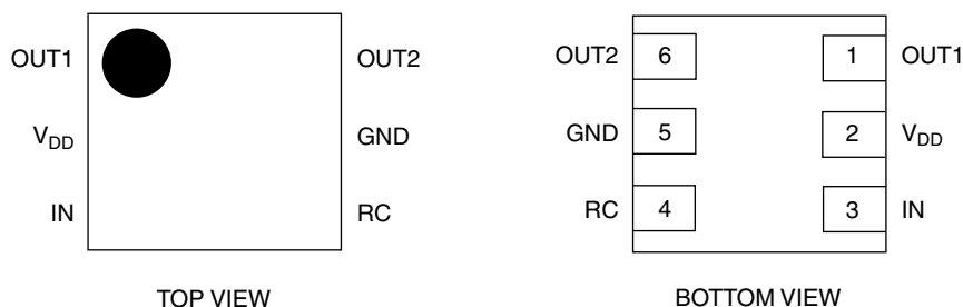
SC89 PACKAGE
