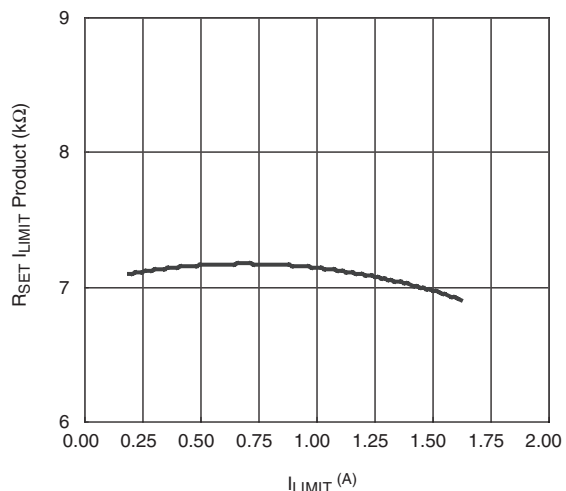
R_{SET} Coefficient vs. I_{LIMIT}
