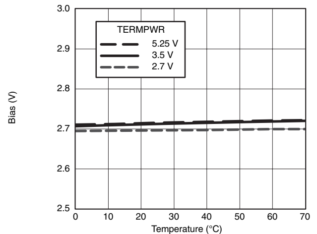
Bias vs. Temperature
