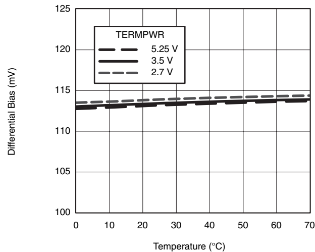
Differential Fail-Safe Bias vs. Temperature
