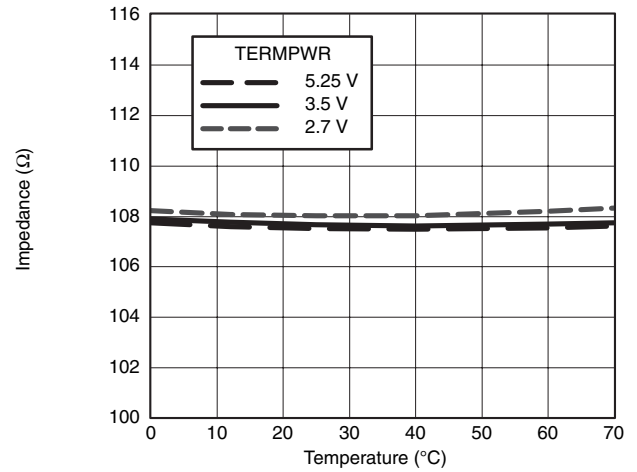
Impedance vs. Temperature
