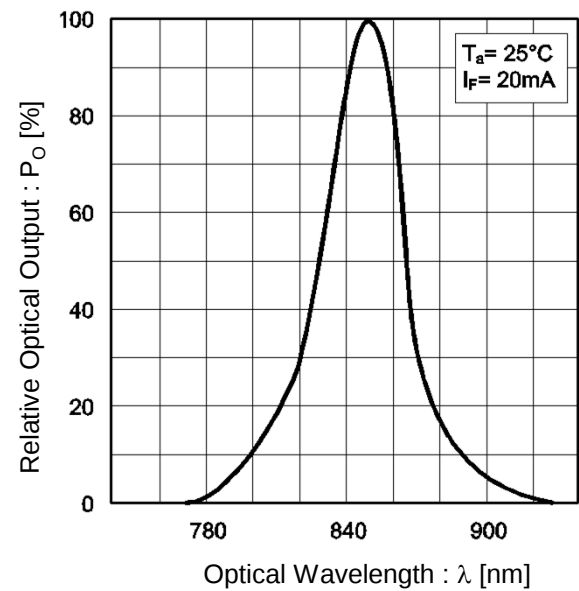
Fig.3 Wavelength
