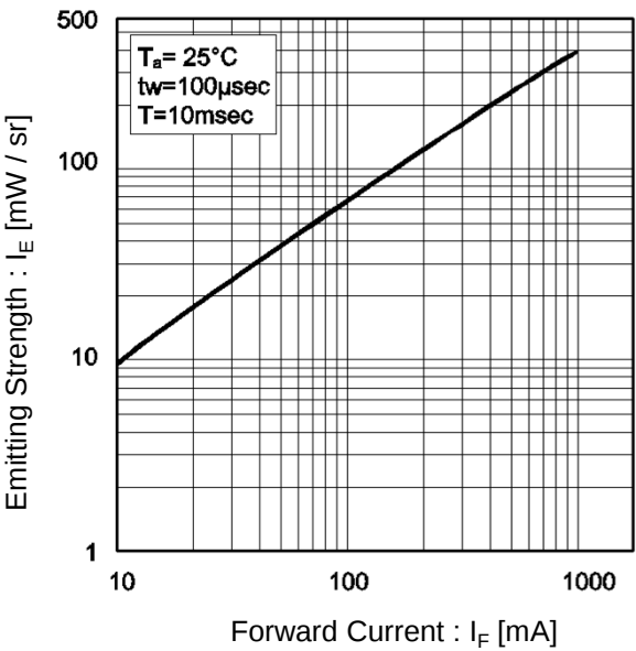
Fig.4 Emitting Strength vs. Forward Current
