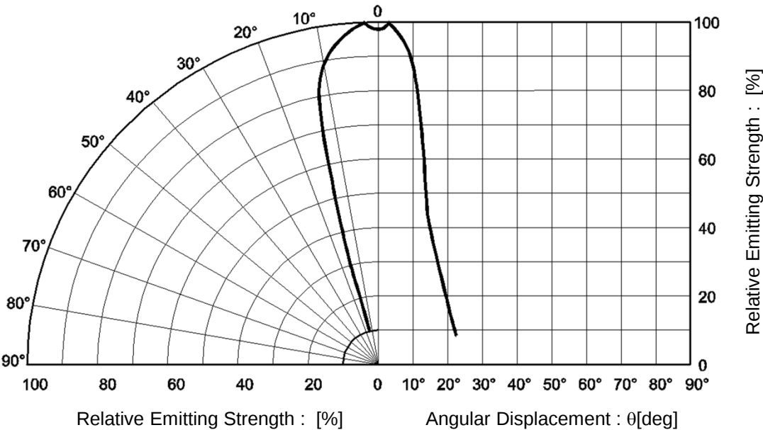
Fig.7 Directional Pattern
