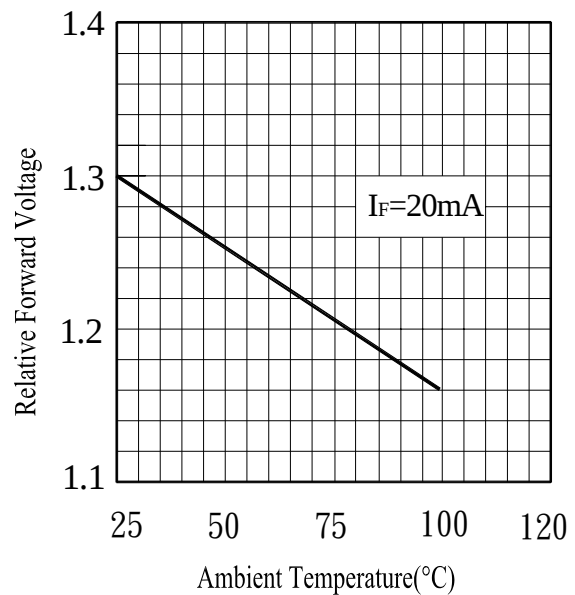
Fig.8 Forward Voltage vs. Ambient Temperature( ^\circ C)
