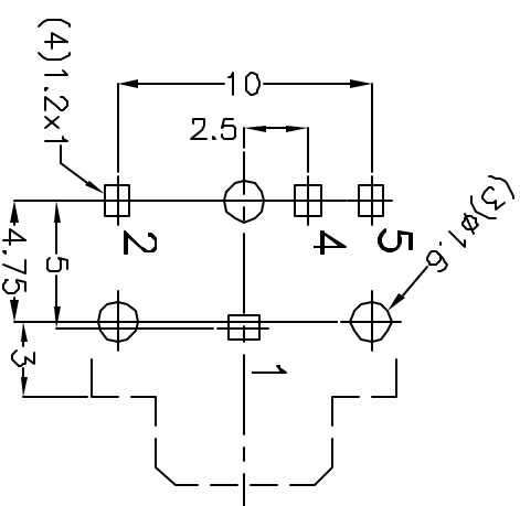
HOLE LAYOUT (TOP VIEW)
