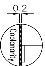
Mounting Surface
