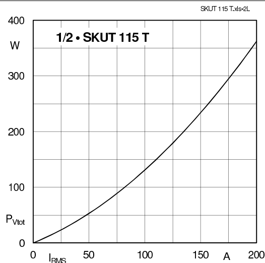
Fig. 2: Power dissipation per thyristor vs r.m.s. current
