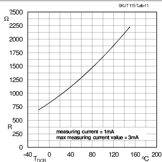
Fig. 11: Temperature sensor characteristic
