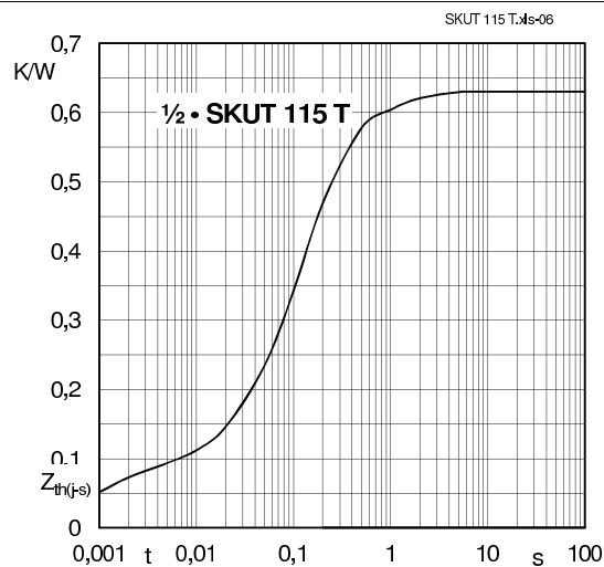
Fig. 6: Transient thermal impedance Z_{th(j-s)}
