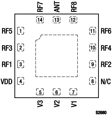
Figure 2. SKY13418-485LF Pinout – 14-Pin QFN (Top View)
