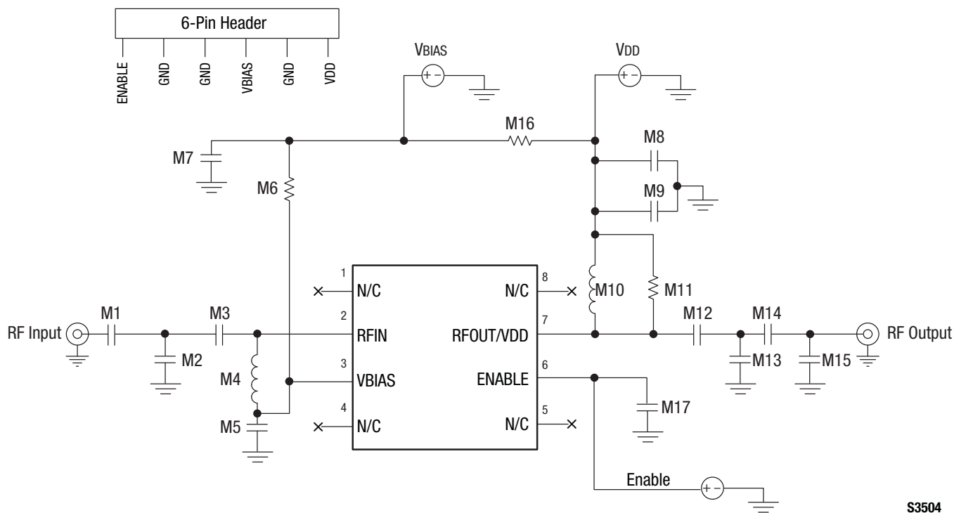
Figure 25. SKY67153-396LF Evaluation Board Schematic (700 to 3800 MHz)
