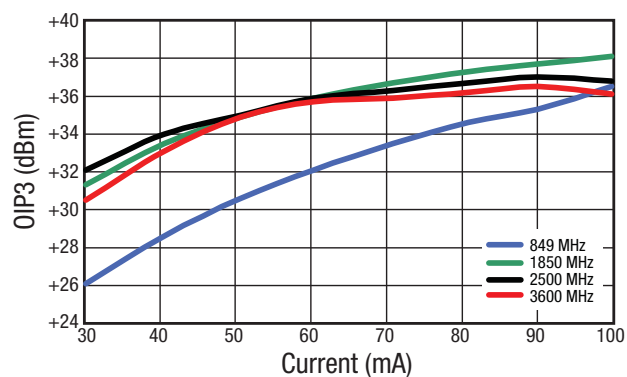
Figure 16. OIP3 vs Quiescent Current over Frequency Using Band-Specific BOM
