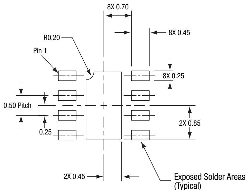
Figure 26. SKY67153-396LF PCB Layout Footprint (Top View)
