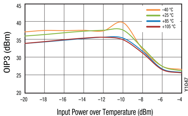
Figure 15. OIP3 vs Input Power over Temperature (@2500 MHz, 1MHz Spacing)
