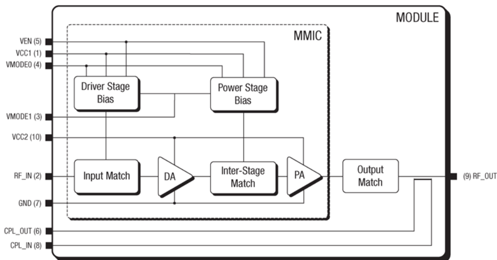
FIGURE 1. SKY77761-12 FUNCTIONAL BLOCK DIAGRAM
