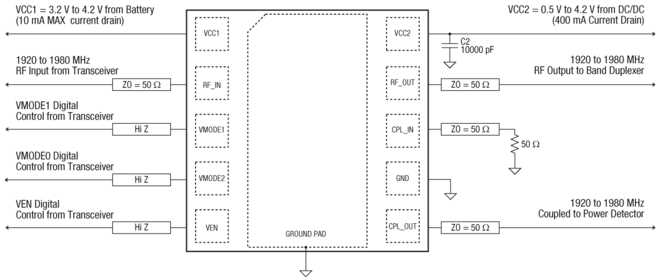
FIGURE 4. SKY77761-12 SCHEMATIC FOR RECOMMENDED APPLICATION DIAGRAM
