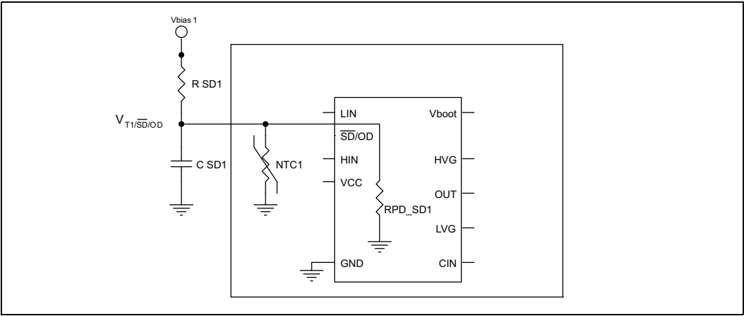
Figure 4. Internal structure of \overline{\text{SD}} and NTC (a)
