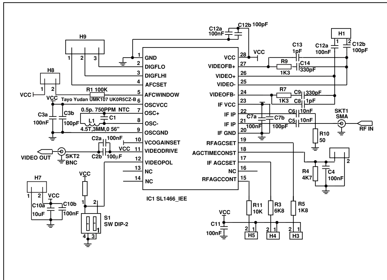
Fig. 6 Typical application circuit.
