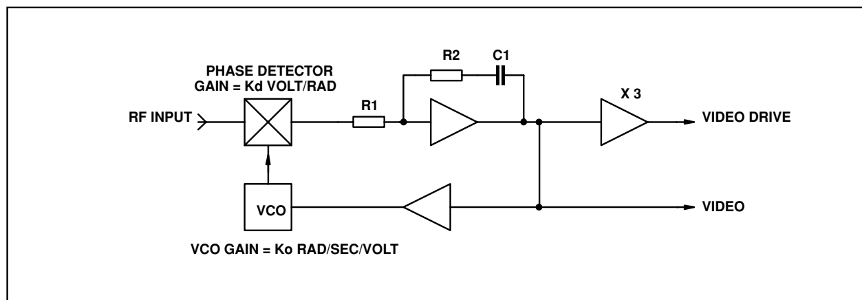
Fig. 3 Design of PLL loop parameters
