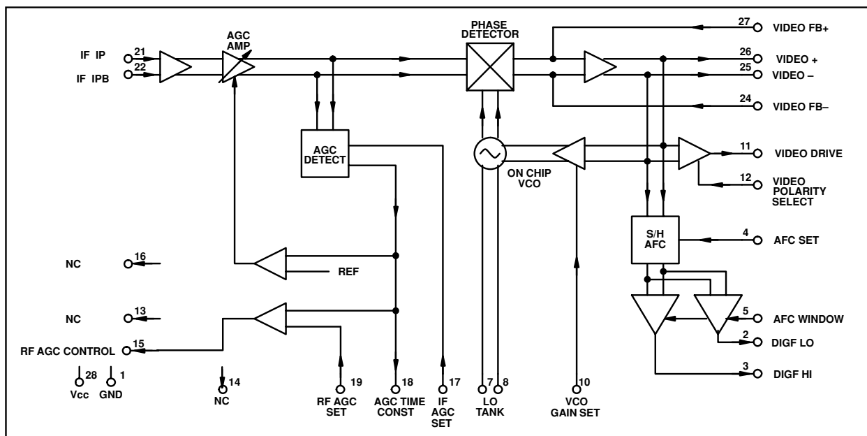
Fig. 2 Block diagram
