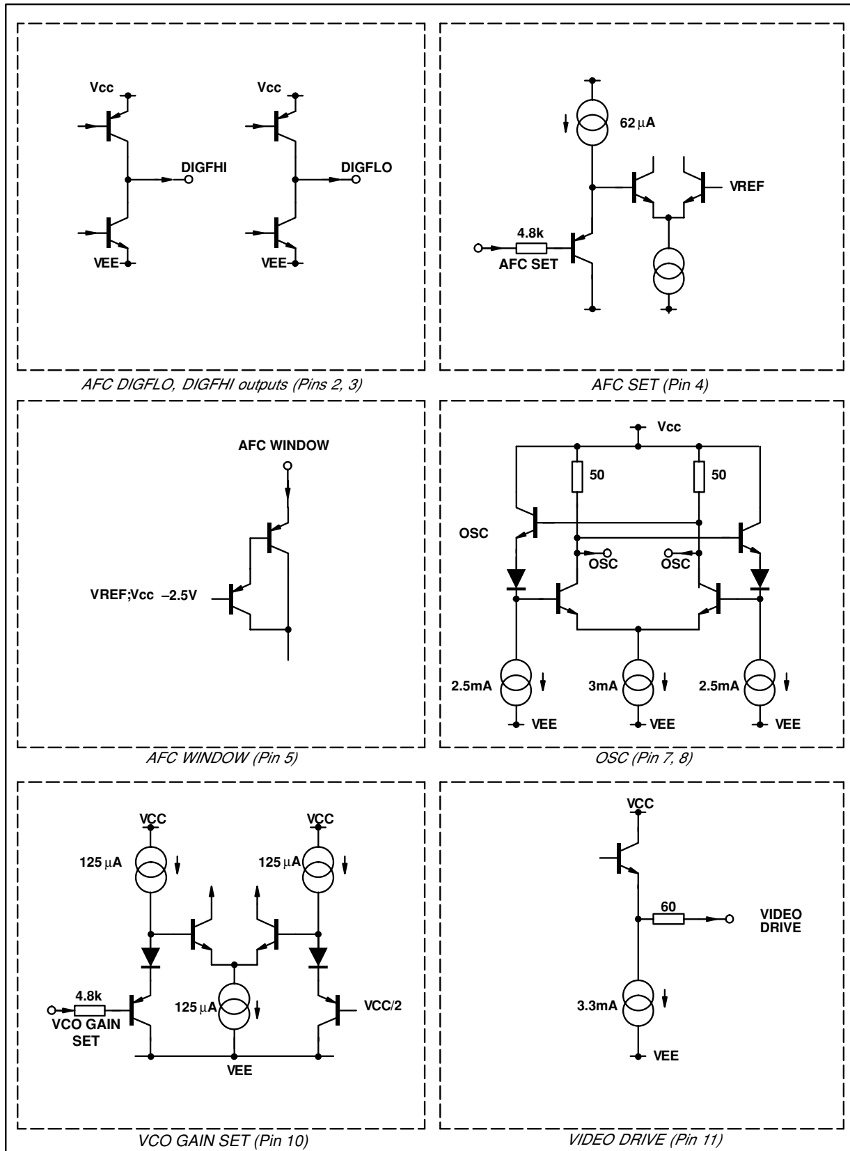
Fig. 5a SL1466 I.O.ports internal circuitry
