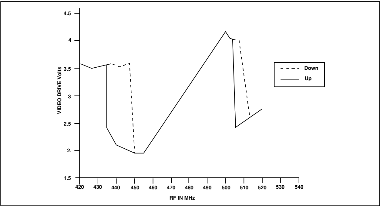
Fig.8 VCO performance (S curve characteristics)
