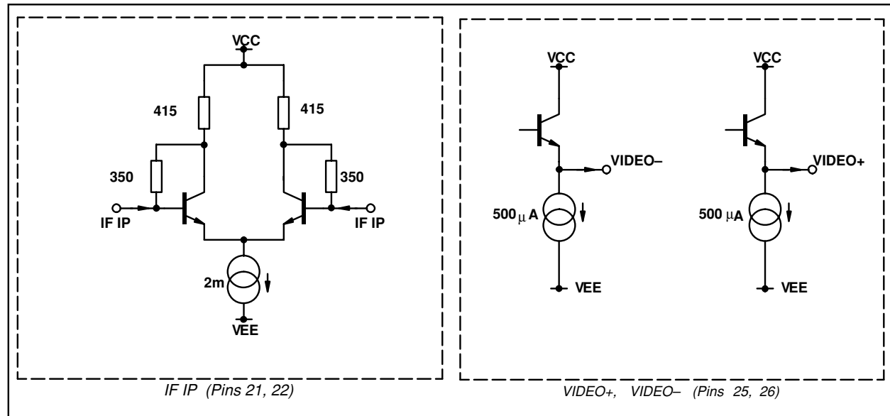
Fig. 5c SL1466 I.O ports internal circuitry
