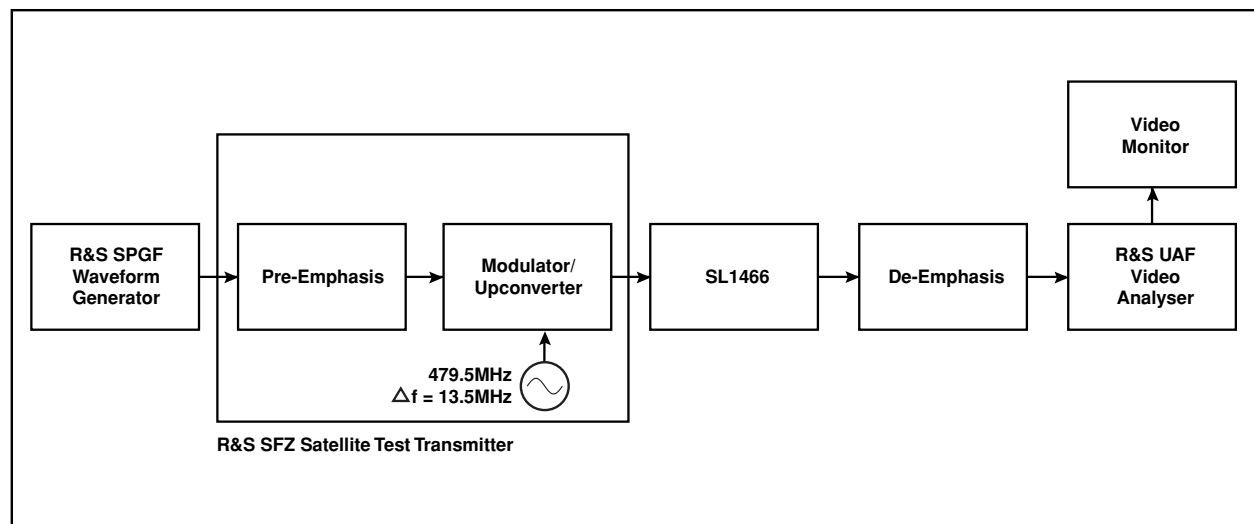
Fig. 11 Test set up
