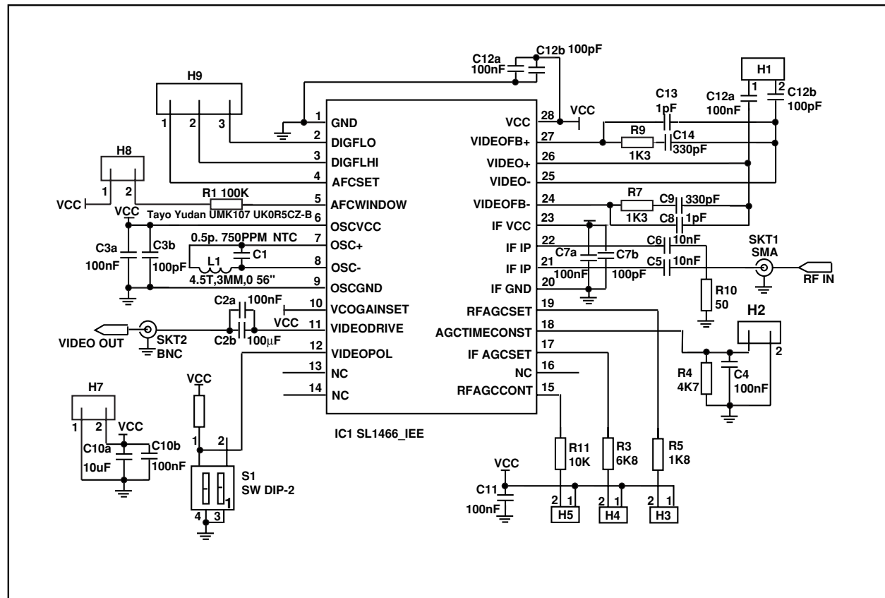
Fig. 10 Test/Demo circuit diagram
