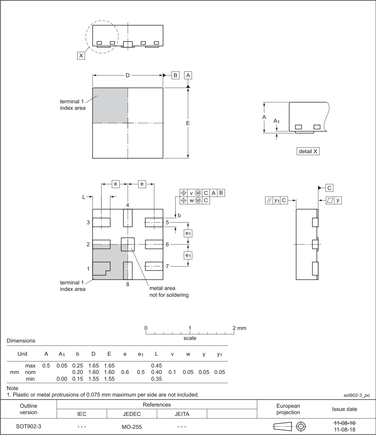
Fig 9. Package outline SOT902-3
