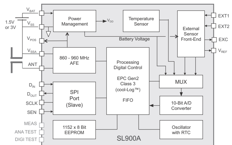
Figure 10: Block Diagram
