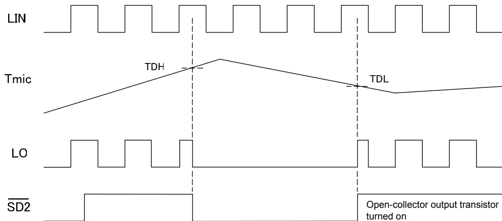
Low-Side Logic TSD Timing Diagram
