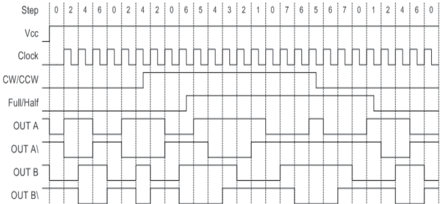
Timing chart
