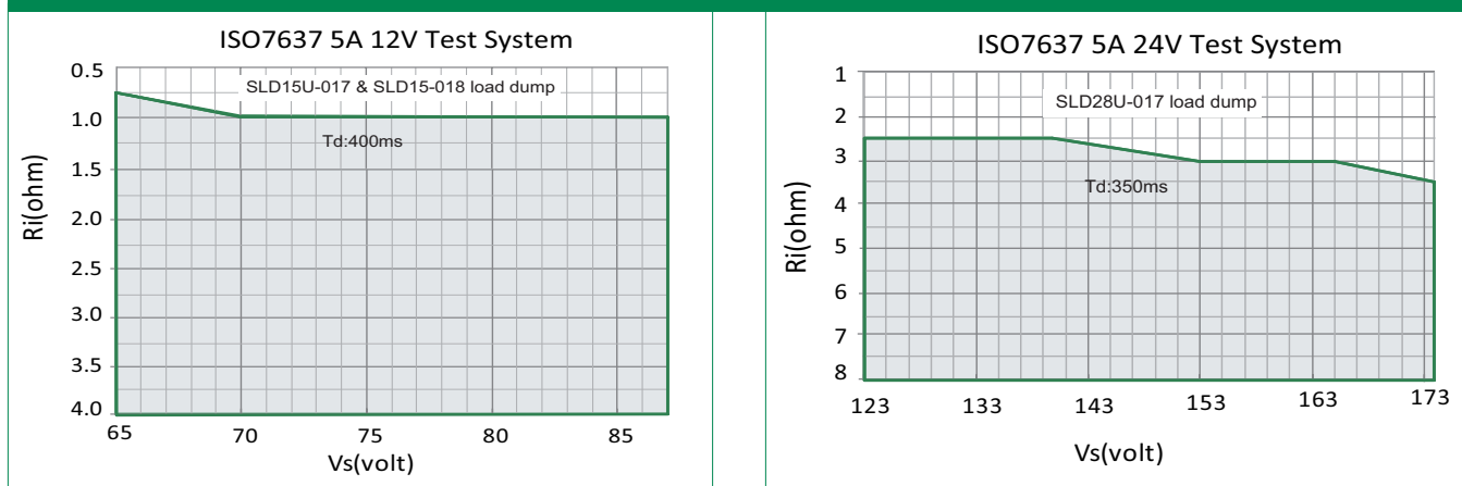
Figure 7 - SOA Chart
