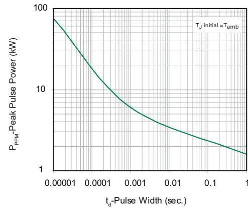
Figure 2 - Peak Pulse Power Rating Curve
