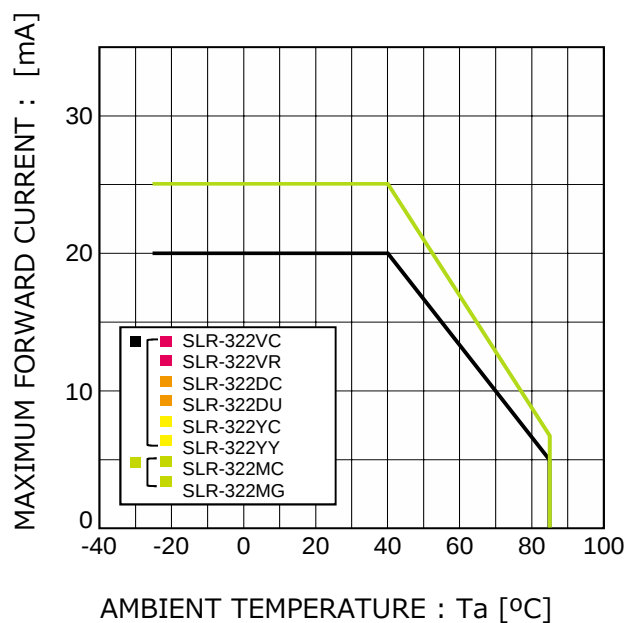
Fig.4 Derating
