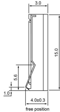
SIDE VIEW (1)
