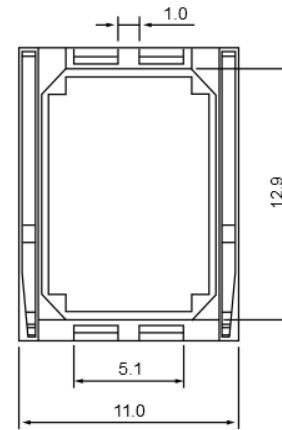
BOTTOM VIEW
