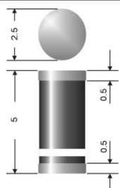
Surface mount diode
