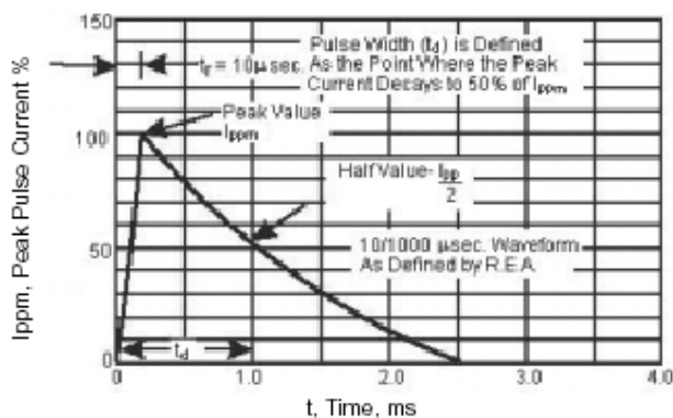
Clamping Power Pulse waveform
