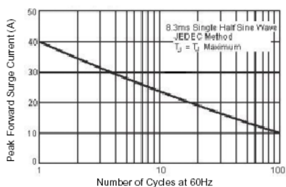
Maximum Non-Repetitive Peak Forward Surge Current
