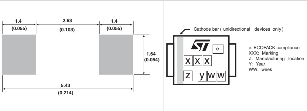
Figure 13. Footprint dimensions in mm (inches)
