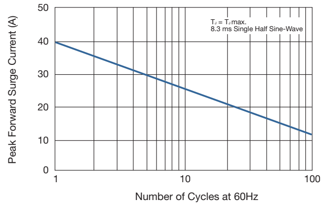
FIG 2. MAXIMUM NON-REPETITIVE
