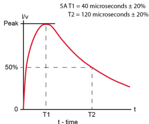
FIGURE 9 – Waveform 5A
