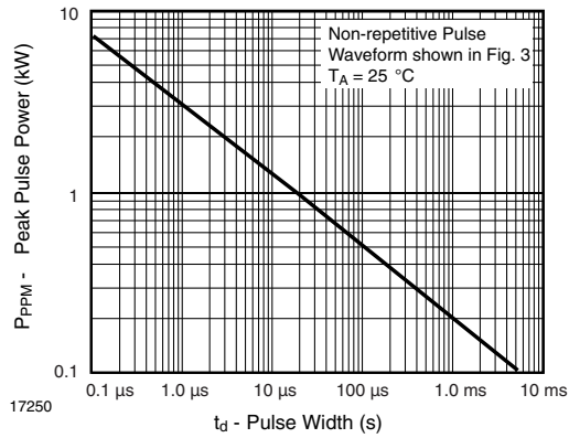
Figure 1. Peak Pulse Power Rating
